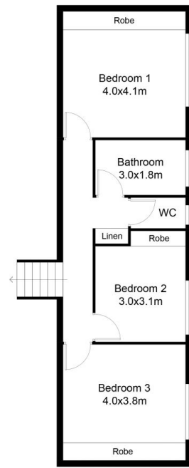
Upper Floor
