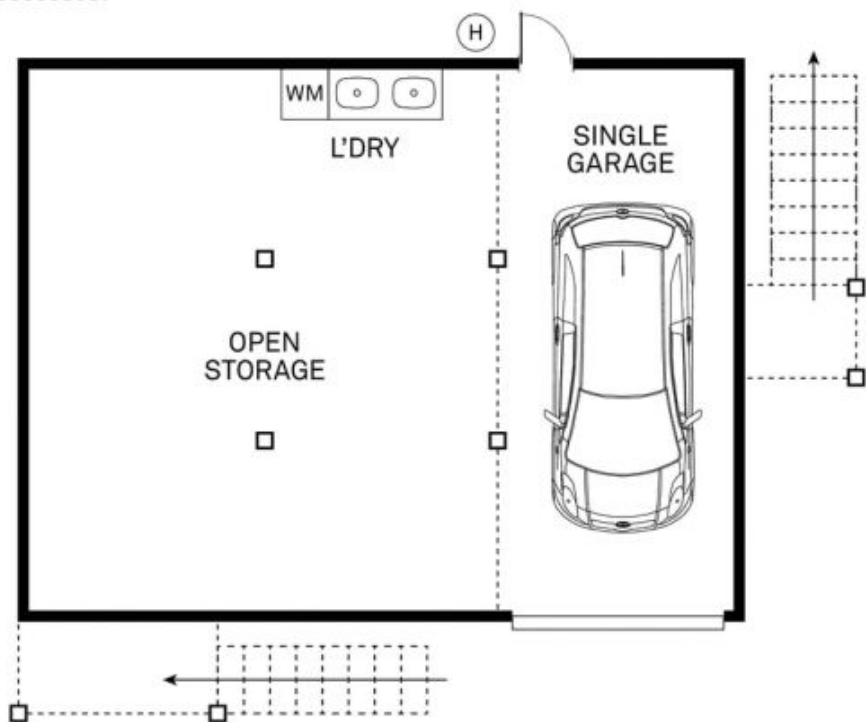
LOWER FLOOR
